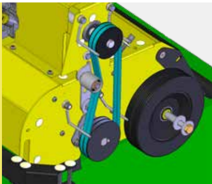
Double-belt transmission.
